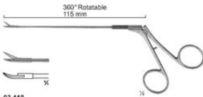
03-118 CASPAR Micro Scissor Curved Size: 115 mm
